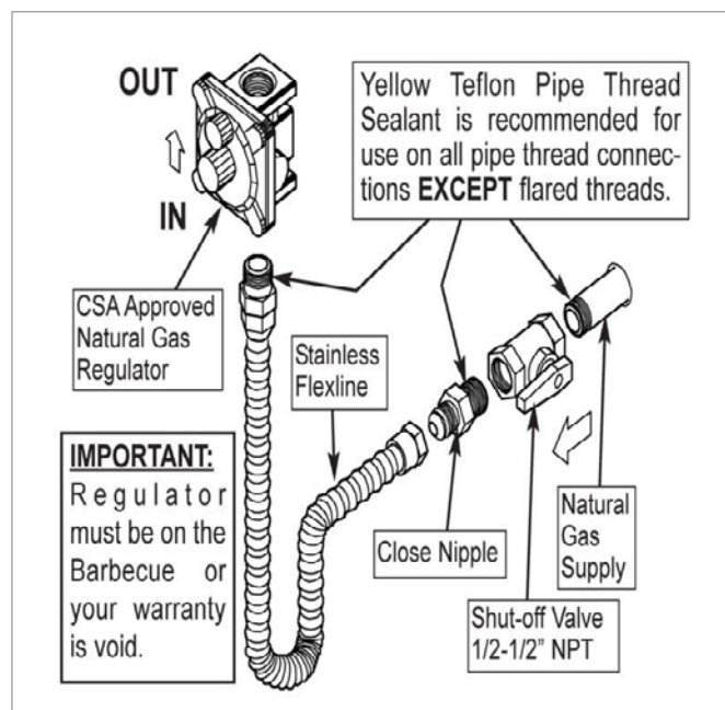
Installation Method for Low Pressure Gas Source – (Natural Gas Regulator Shown)
