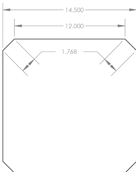
TF-NK-15D ISLAND TOP VIEW CUTOUT DIMENSIONS
