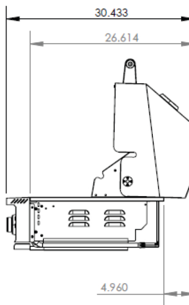
TF25, TF30, & TF42 HOOD CLEARANCE
